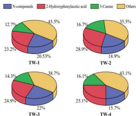
Figure 4. The main products of tobacco wastes during purge/trap-GC/MS.
